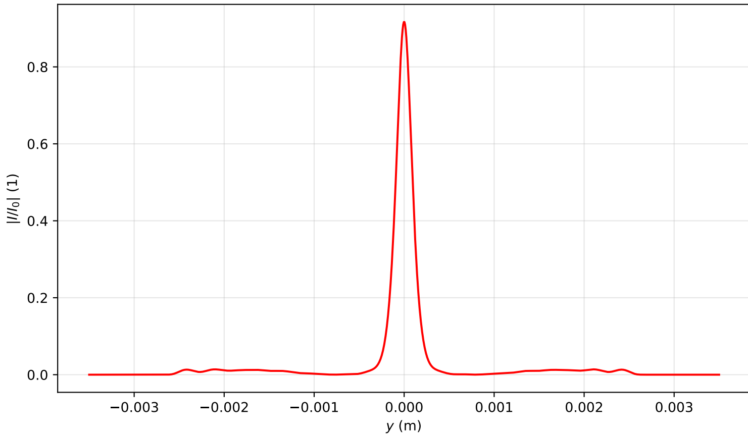
Intensity profile I(x=0, y, z=2.070)/I_0 , P_{in}=9.0P_{cr} , artificial time
